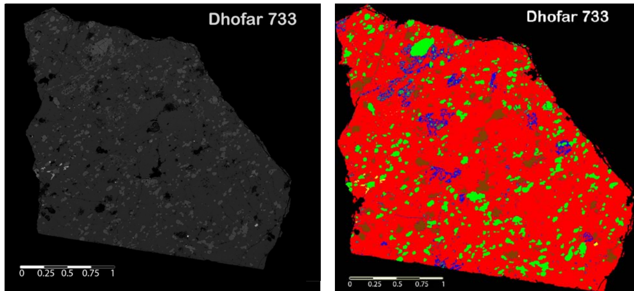
Figure 1. (a) Back-scattered electron (BSE) mosaic of Dhofar 733. Scale in mm. (b) False-color image of Dhofar 733. Red = Plagioclase/Maskelynite, Green = Olivine, Blue = Pyroxenes, Yellow = Oxides, Brown = Fractures. Scale in mm.
