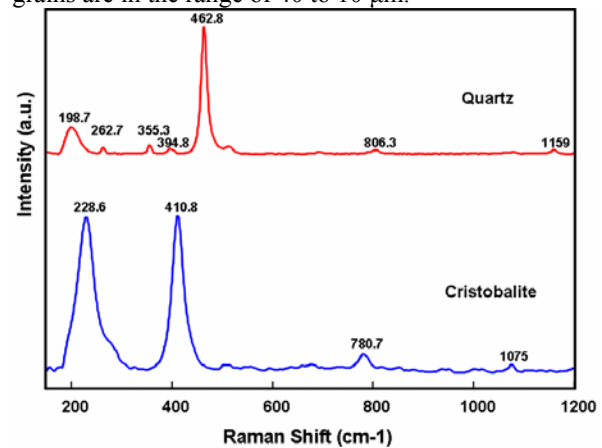
Figure 2. Raman spectra of quartz and cristobalite.
